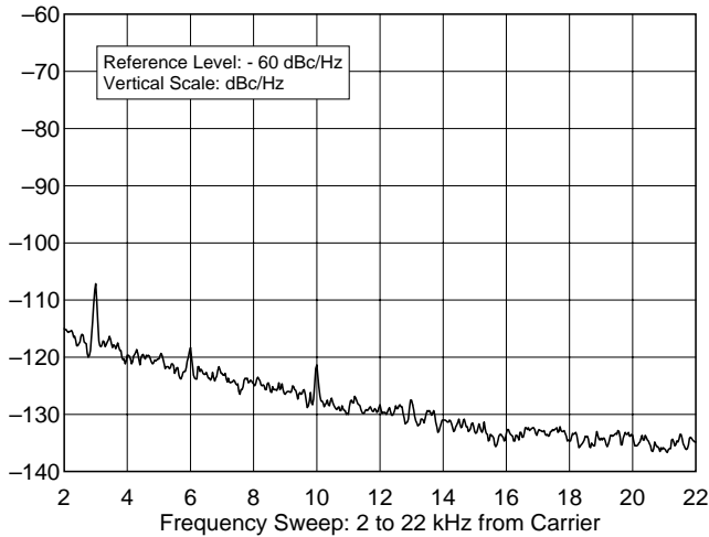
ICOM IC-746 Pro, s/n 01484 50.020 MHz, Phase Noise: 100 W I:\PRODREV\TESTS\IC746PRO\746PRP6M.TXT
