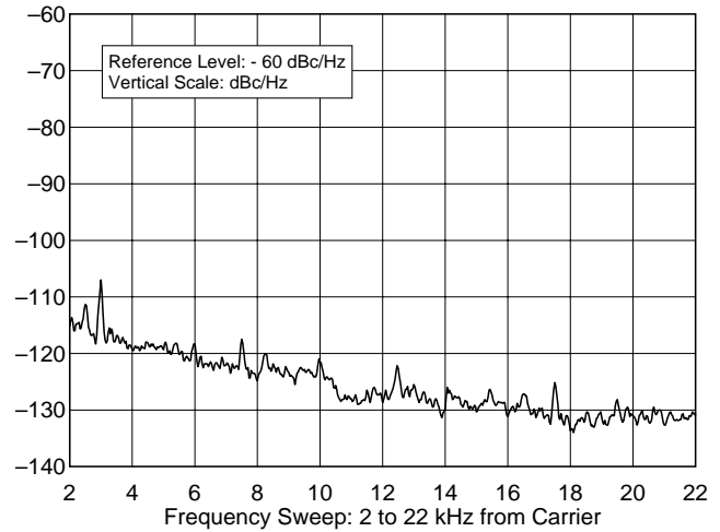
ICOM IC-746 Pro, s/n 01484 144.020 MHz, Phase Noise: 100 W I:\PRODREV\TESTS\IC746PRO\746PRP2M.TXT
