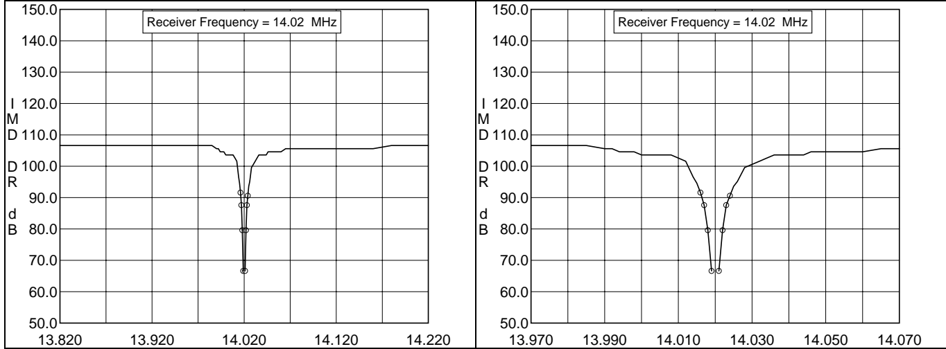
IMD Dynamic Range, Preamp Off
